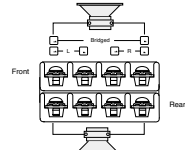
1-channel configuration
