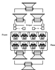
3-channel configuration
